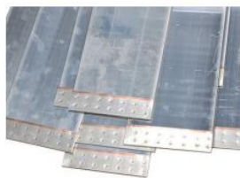
880KVA MFDC Double Heads Spot Welder for Aluminum Bus Bar DB-880-15001
